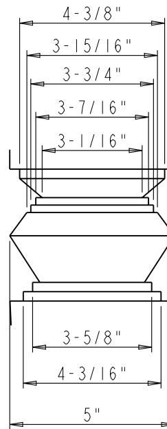
DETAIL A SCALE 1:4
