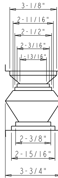
DETAIL A SCALE 1:4
